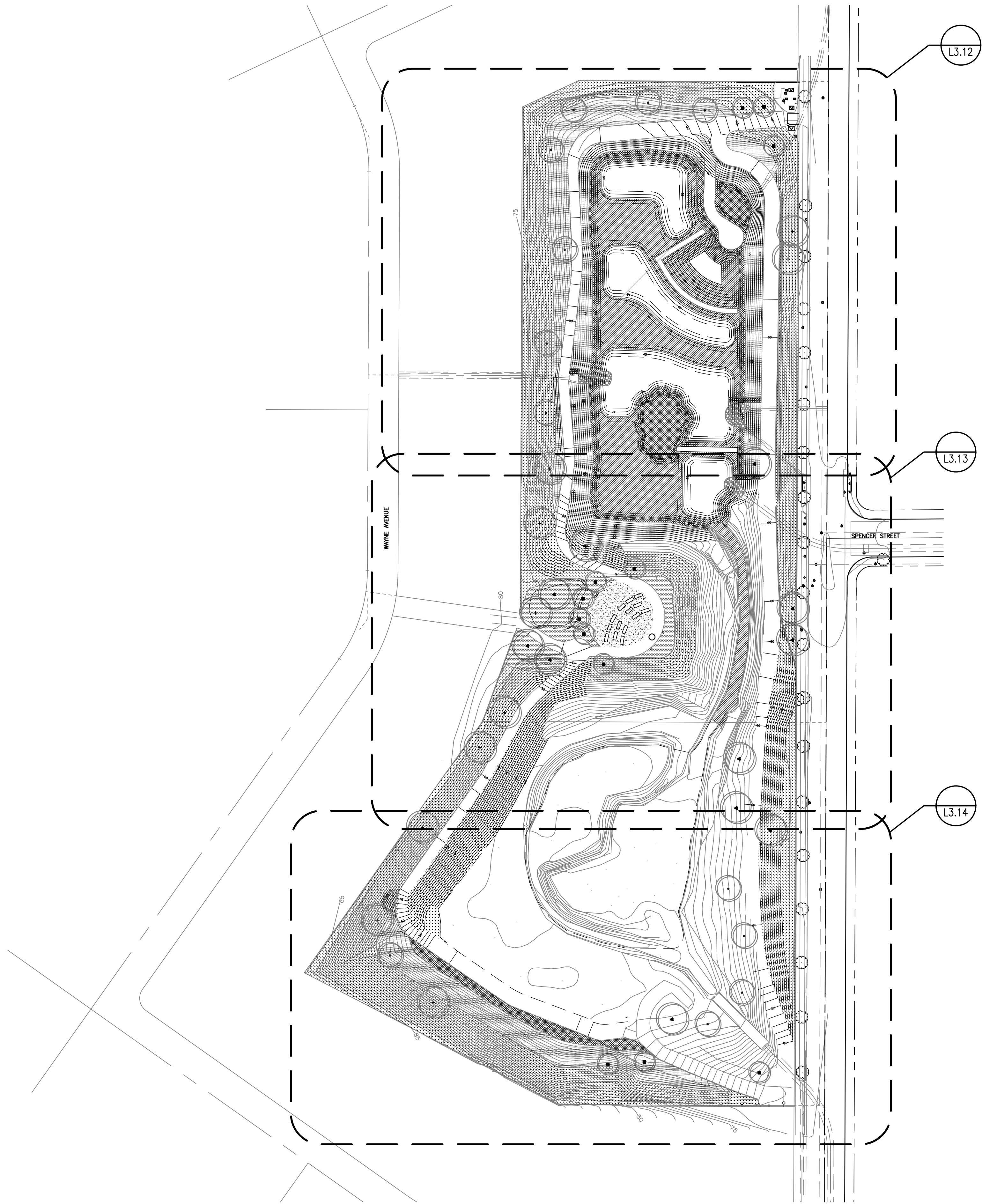
1 HENRIETTA BASIN - OVERALL PLANTING PLAN SCALE: 1" = 60'
